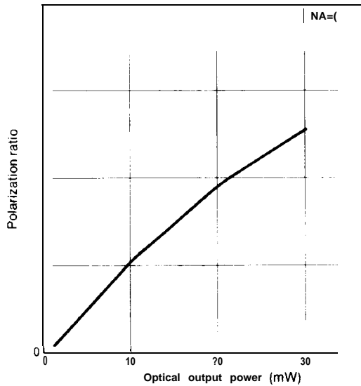
Fig. 94-3 Polarization Ratio vs. Optical Power Output (LT024 series, LTO15 series)
