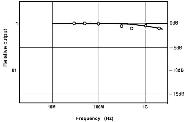
Fig. 94-5 Frequency Response
